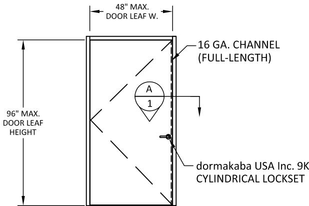
OUTWSWING SINGLE STEEL DOOR DOORS UNDER SEPARATE APPROVAL
